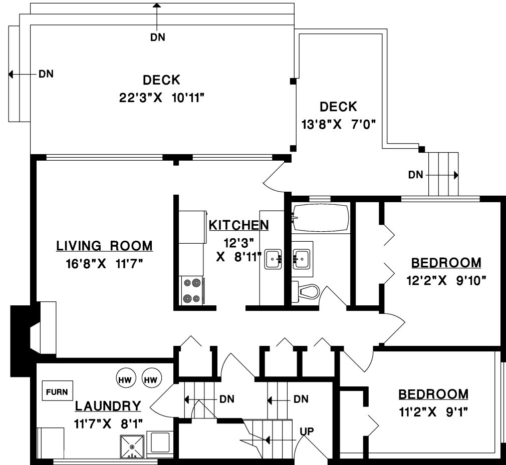
LOWER FLOOR
