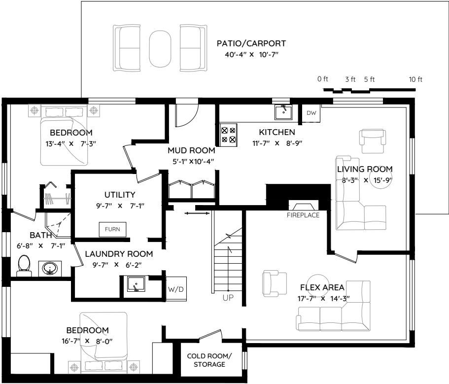
LOWER FLOOR 1,311 SQ.FT. CH: 7'-7"
