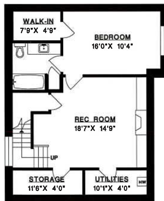
LOWER FLOOR
