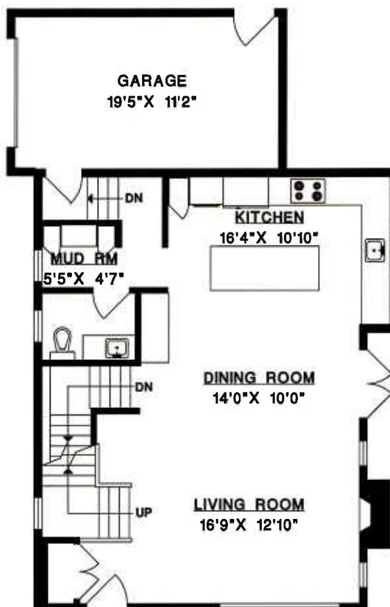
MAIN FLOOR
