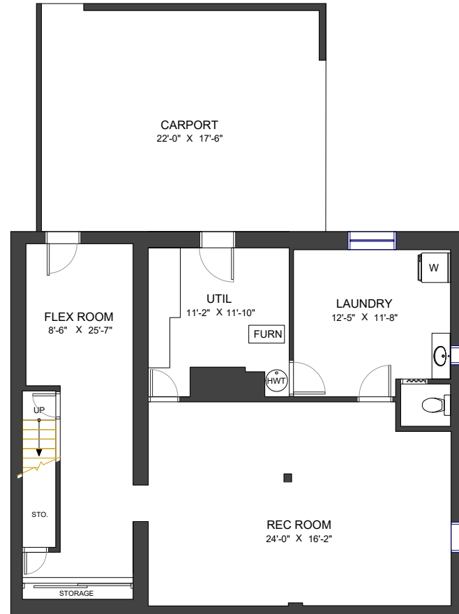
Lower Floor Ceiling Height: 7'
