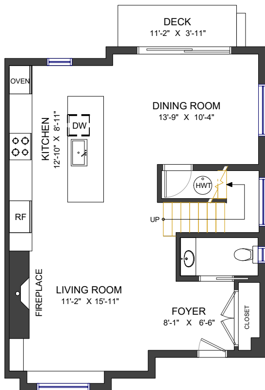
Main Floor Ceiling Height: 9'
